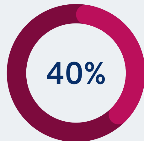
Statistic 1
