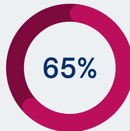
Statistic 2
